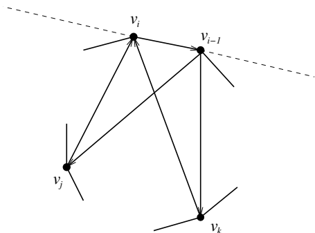
Figure 1.1. A convex polygon.
