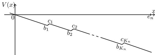
Figure 3.1. Potential and valleys.
