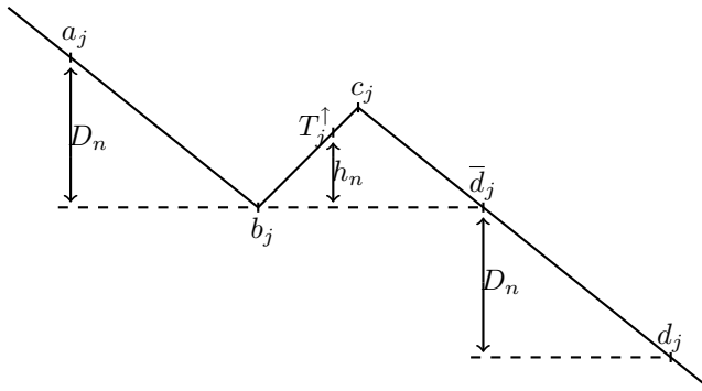
Figure 3.2. Zoom on the j -th valley.
