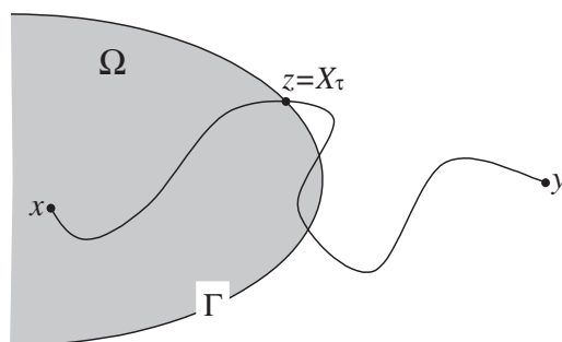
Figure 6. A path between points x, y
