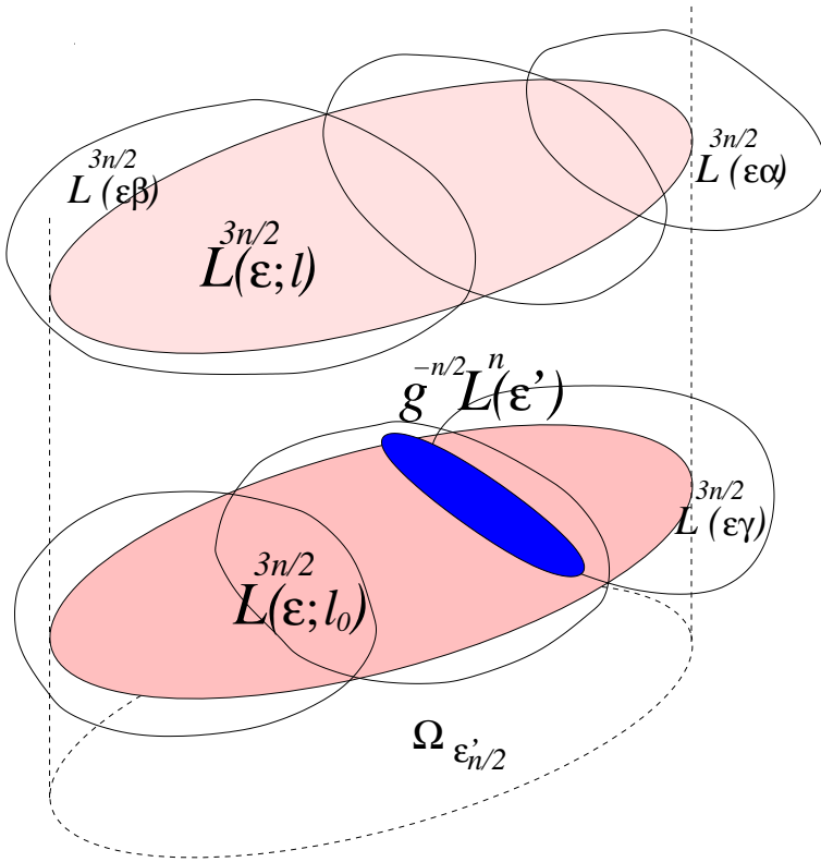
Figure 3.2. Decomposition of (g^{n/2} \mathcal{L}^n(\epsilon)) \cap T^* \Omega_{\epsilon'_{n/2}} into connected leaves (here we show two of them, in light grey). The leaf \ell contains the components \mathcal{L}^{\frac{3}{2}n}(\epsilon\alpha) , \mathcal{L}^{\frac{3}{2}n}(\epsilon\beta) while the leaf \ell_0 contains \mathcal{L}^{\frac{3}{2}n}(\epsilon\gamma) . We also show the elongated leaf g^{-n/2} \mathcal{L}^n(\epsilon') supporting the state w^{n/2}(\epsilon') (black). This state might interfere with v^{\frac{3}{2}n}(\epsilon, \ell_0) , but not with v^{\frac{3}{2}n}(\epsilon, \ell) or any other leaf above \Omega_{\epsilon'_{n/2}} .
