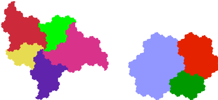
Figure 5.2. Central tile for the \beta -substitution associated with the smallest Pisot number \sigma_3 and the Tribonacci substitution \sigma_4 . Their inverse automorphisms are not Pisot and cannot be represented by a central tile.
