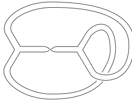
Figure 1.5. A Möbius graph.
