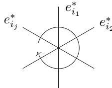
Figure 2.1. A j -valent vertex with a cyclic order given to incident half-edges. Each half-edge is labeled by i_k , and an element e_{i_k}^* is assigned.
