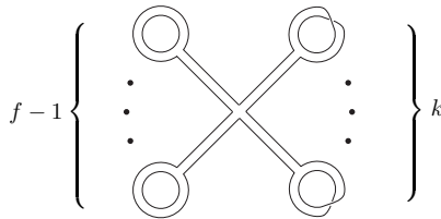
Figure 3.2. A standard graph for a non-orientable surface of topological type (k, f) . It has f - 1 tadpoles on the left, and k twisted tadpoles on the right.
