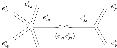
Figure 3.1. A half-edge labeled by i_3 of the left vertex is connected to a half-edge labeled by j_3 of the vertex at the right by a twisted edge. A propagator \langle e_{i_3} e_{j_3}^* \rangle is assigned to this edge.
