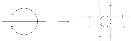
Figure 1.1. A vertex with a cyclic order given to incident half-edges. It is placed on a plane with the clockwise orientation. The half-edges become crossroads with a compatible orientation at the boundary.
