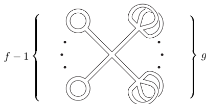
Figure 2.3. A standard graph of topological type (g, f) . It has f - 1 tadpoles on the left, and g bi-petal flowers on the right.
