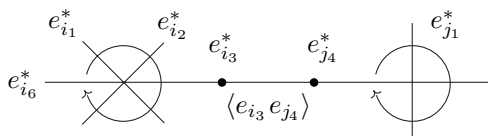
Figure 2.2. A half-edge labeled by i_3 of the left vertex is connected with a half-edge labeled by j_4 of the vertex at the right. A propagator \langle e_{i_3} e_{j_4} \rangle is assigned to this edge.
