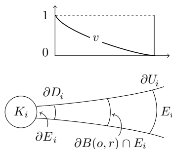
Figure 9. Manifold M_i and function v in U_i \setminus \bar{D}_i
