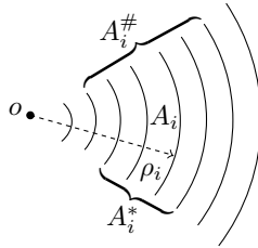
Figure 3. A good covering by annuli
