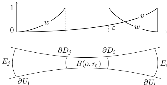
Figure 10. Functions v and w
