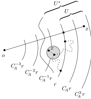
Figure 7. Any point x \in U^* can be connected to a point on \partial B(o, r) by a curve in U^* (the shaded ball has radius s )
