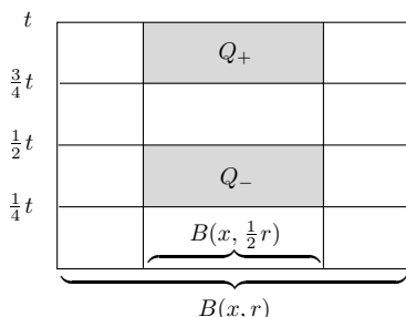
Figure 1. Cylinder Q = (0, t) \times B(x, r)
