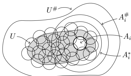
Figure 2. A good covering by balls
