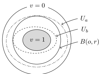
Figure 8. Sets U_a and U_b
