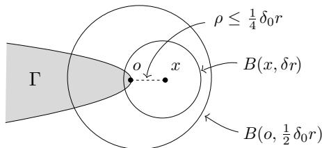
Figure 4. The balls B(o, \frac{1}{2} \delta_0 r) and B(x, \delta r)
