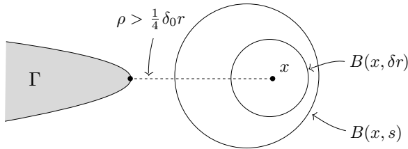
Figure 5. Remote ball B(x, s) and the ball B(x, \delta r) = B(x, \delta_0 s)
