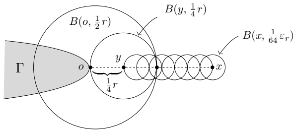
Figure 6. Comparisons of \mu(B(x, \frac{1}{64}\varepsilon r)) and \mu(B(y, \frac{1}{4}r))
