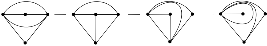
Figure 2.14. Modifying \gamma_0 to avoid a before u'
