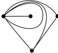
Figure 2.13. The local behavior of the triangulation u'
