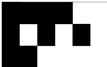
Figure 8.7. A tile T with \pi_1(T) = \mathbb{Z} .
