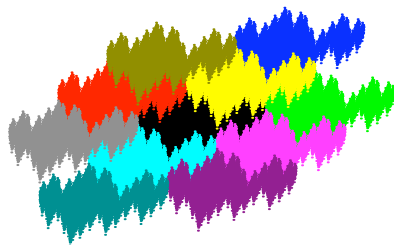
Figure 8.3. The tile \mathcal{T}_2 and its neighbors.
