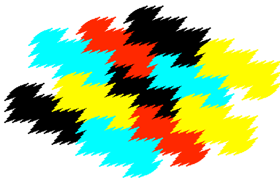
Figure 8.1. The tile T_1 and its neighbors.
