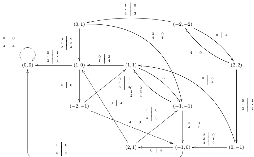
Figure 8.5. The graph G^T(S_3) ( L is an abbreviation for d|d - 2, 2 \leq d \leq 4 ).
