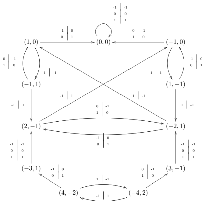
Figure 8.1. The tile T_1 and its neighbors.
