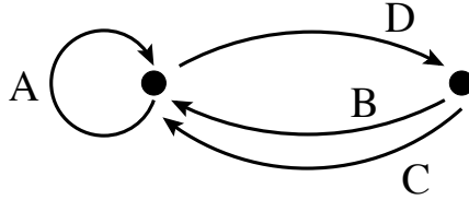
Figure 5.1. A topological representation of \varphi_4 (the inverse of the Tribonacci substitution) given by the graph G_4 provided with the map A \mapsto DC , B \mapsto D^{-1}A , C \mapsto B , D \mapsto C^{-1} .
