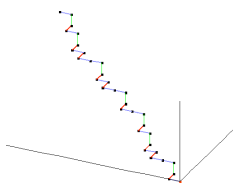
Figure 4.1. The discrete line \mathcal{D}_\sigma
