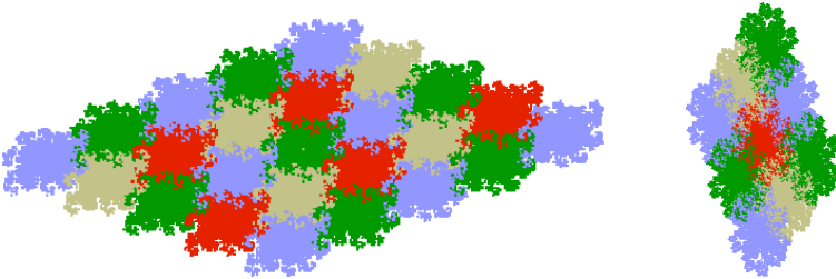
Figure 4.5. Left side: the periodic tiling generated by \varphi_1 : a \mapsto c, b \mapsto c^{-1}a, c \mapsto b on F_3 ; \varphi_1 induces an irreducible unit Pisot nonorientable train-track map. Each tile intersects exactly six neighbours; the intersection has zero measure. Right side: The central tile of \varphi_2 : a \mapsto c, b \mapsto c^{-1}a, c \mapsto bc^{-1} also periodically tiles the plane, but each tile has eight neighbours.
