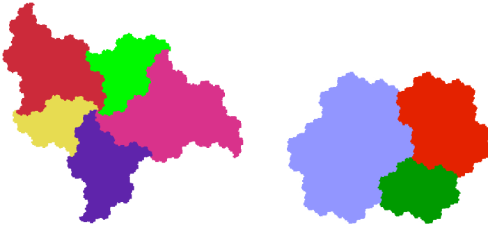
Figure 5.2. Central tile for the \beta -substitution associated with the smallest Pisot number \sigma_3 and the Tribonacci substitution \sigma_4 . Their inverse automorphisms are not Pisot and cannot be represented by a central tile.
