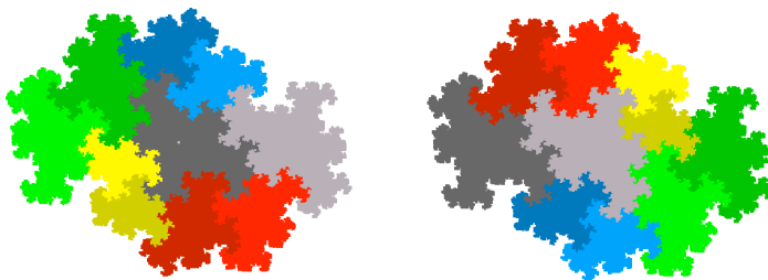
Figure 5.4. Exchange of domains for the central tile \varphi_6 . It has 10 subtiles.
