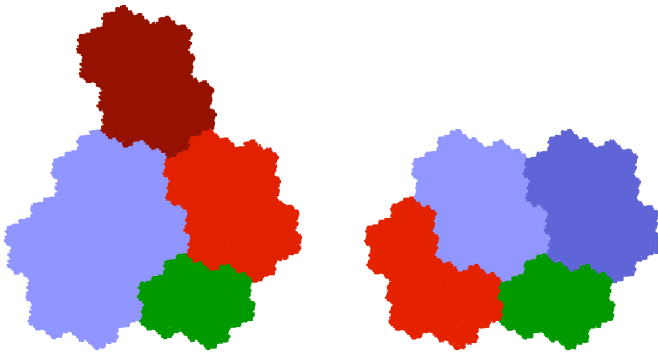
Figure 6.2. Relations between central tiles for conjugate substitutions. Left side: the basic subtiles of \mathcal{T}_{\tau_4} (central tile of \tau_4 ) can be rebuilt from the basic subtiles of \mathcal{T}_{\sigma_4} (central tile of Tribonacci substitution \sigma_4 , conjugate to \tau_4 ). Right side: the basic subtiles of \mathcal{T}_{\sigma_4} can be rebuilt from the basic subtiles of \mathcal{T}_{\tau_4} .
