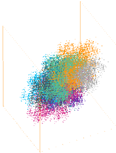
Figure 5.3. Central tile for the train-track map f_5 representing \varphi_5 : it is 3-dimensional, with eight subtiles.
