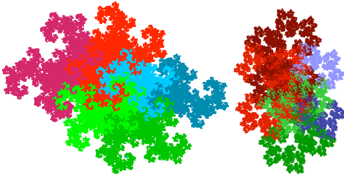
Figure 4.3. Central tiles for \varphi_1 and \varphi_2 (inverse of the flipped Tribonacci substitution).
