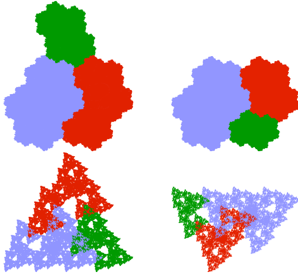
Figure 6.1. Central tiles for two pairs (\tau_4, \sigma_4) , and (\tau_2, \sigma_2) of Pisot unit irreducible substitutions. Each pair consists of substitutions that belong to the same class of automorphisms of F_3 .
