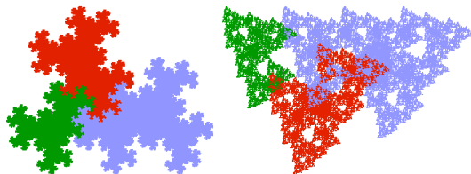
Figure 4.2. Central tiles for the substitutions \sigma_1, \sigma_2 .
