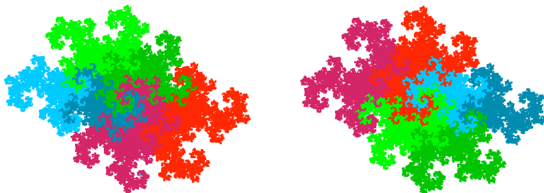
Figure 4.4. Exchange of domains for the central tile of \varphi_1 .
