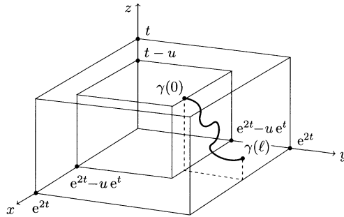
Figure 2. Boxes \Omega_{t,0}, \Omega_{t,u} in the first octant and the path \gamma(s) .
