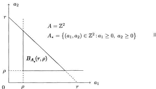
Figure 11. The semigroup A_* has polynomial volume growth of degree 2.
