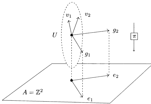
Figure 13. The generating set S of G is the union of \{v_i\} , \{g_i\} and \{g_i^{-1}\} .
