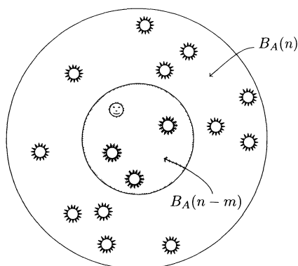
Figure 7. The set \Omega_{n,m} : the lamplighter is inside the ball B_A(n-m) , and the lamps may be “ON” only inside the ball B_A(n) .
