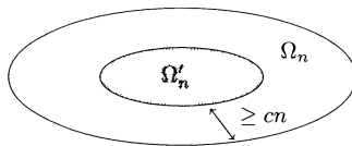
Figure 3. A Følner couple \Omega_n, \Omega'_n .
