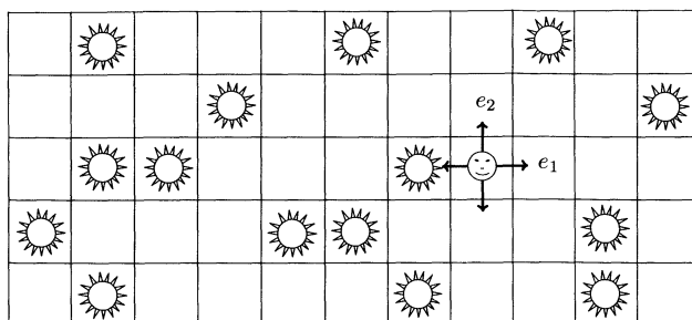
Figure 6. Lamplighter group \mathbb{Z}_2 \wr \mathbb{Z}^2 .
