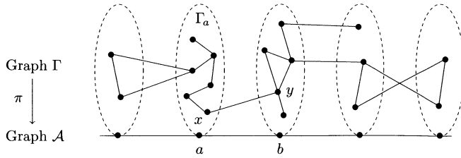
Figure 8. A contraction \mathcal{A} of the graph \Gamma .
