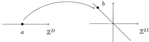
Figure 12. The map a \mapsto b_a .
