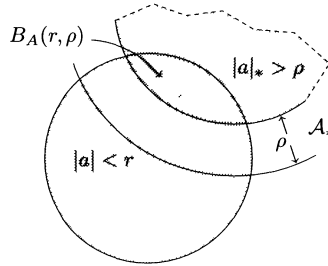
Figure 9. The truncated ball B_A(r, \rho) on \mathcal{A} is the intersection of the sets \{|a| < r\} and \{|a|_* > \rho\} .
