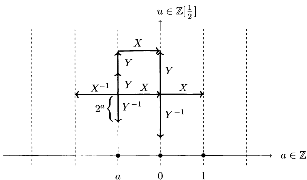
Figure 4. The Cayley graph of the group \mathbb{Z}[\frac{1}{2}] \rtimes \mathbb{Z} .
