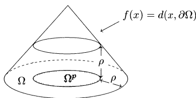
Figure 1. Sets \Omega, \Omega^\rho and function f .
