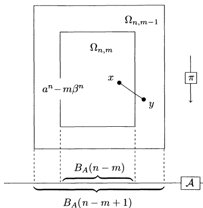
Figure 10. The sets \Omega_{n,m} and \Omega_{n,m-1} in \Gamma .
