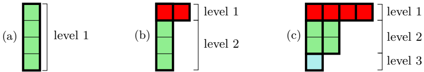
Figure 4.1. Levels (shaded regions) and superboxes (delimited by bold lines) for different Young diagrams: (a) Riemannian, (b) contact, (c) a more general structure.
