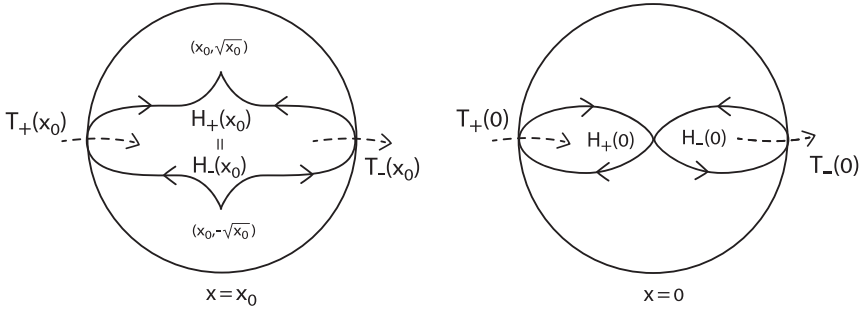
Figure 4.1. Dynamics of \text{Re}(iY)
