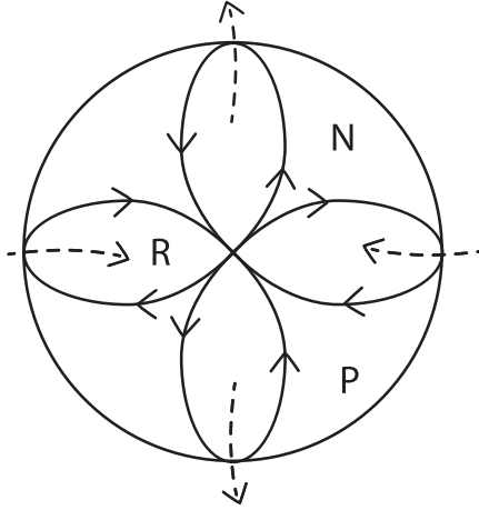
Figure 2.1. Dynamics of \text{Re}(\mu Y)
