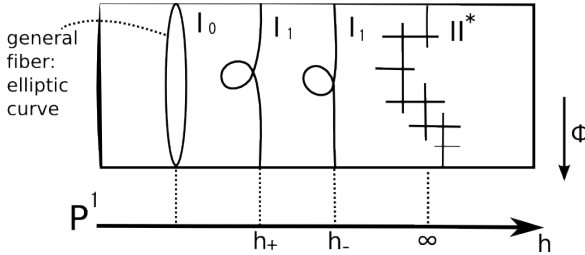
Figure 4.1. The elliptic surface associated to the spectral curves of the autonomous P_1 .
